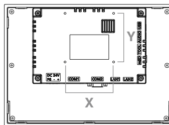
VESA Mount
