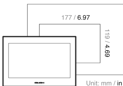
Panel Cut
